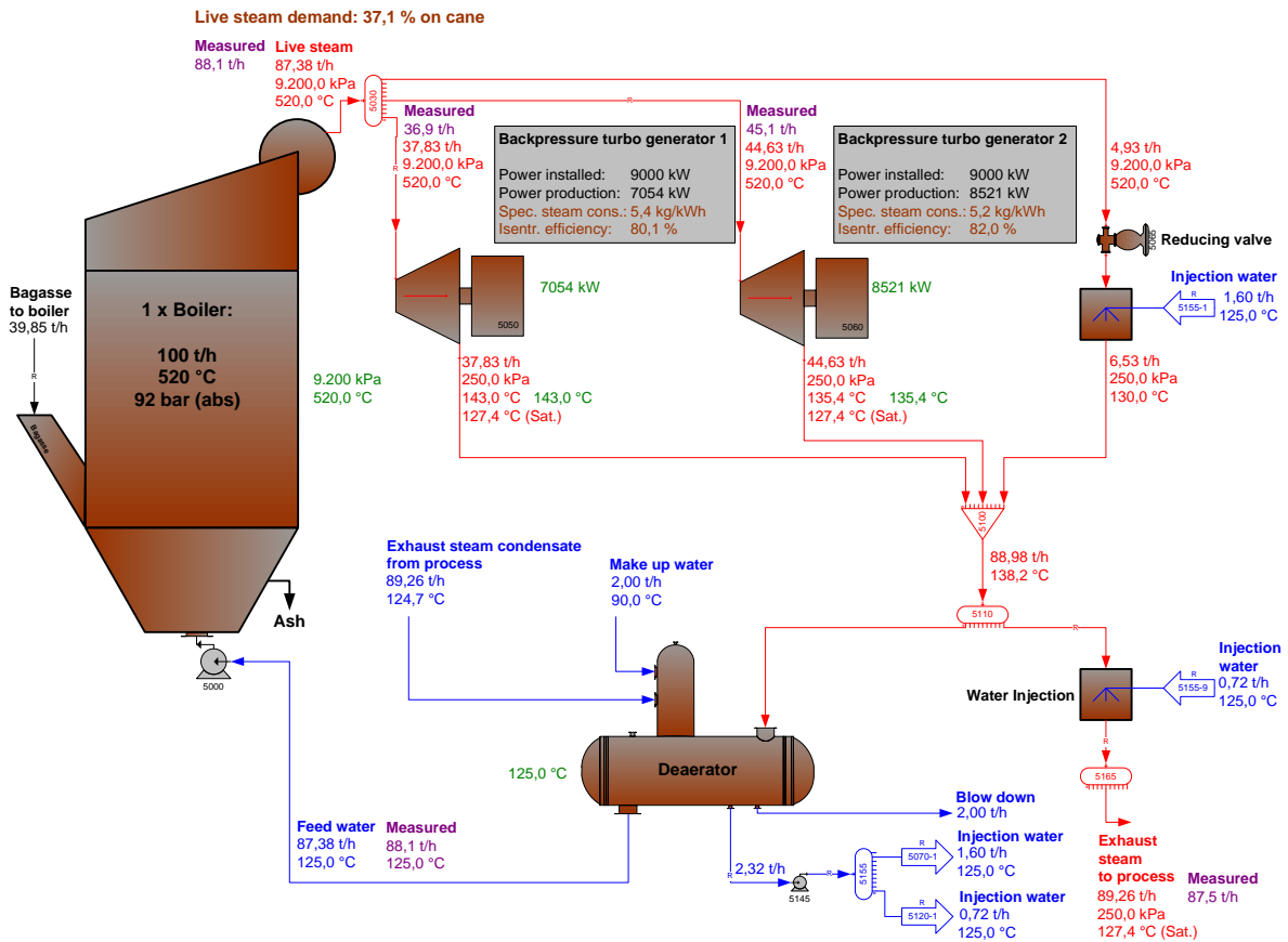
Fig. 4 - Power station simulation
