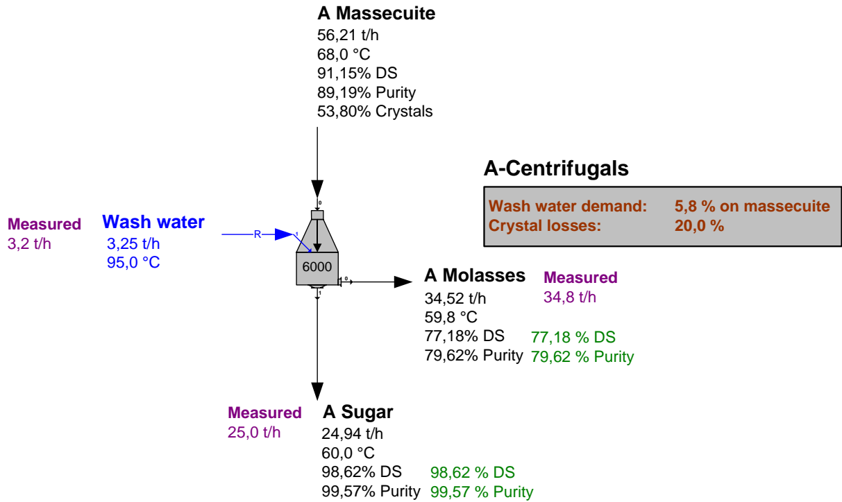
Fig. 3 – Simulation of an A centrifugal station
